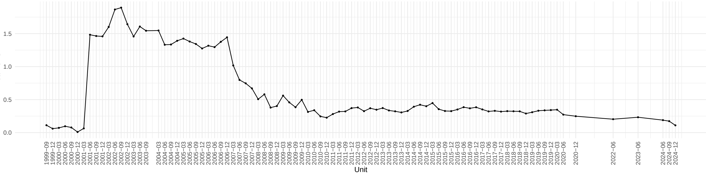
Evolution of HOUSTMW OLS coefficient across time
