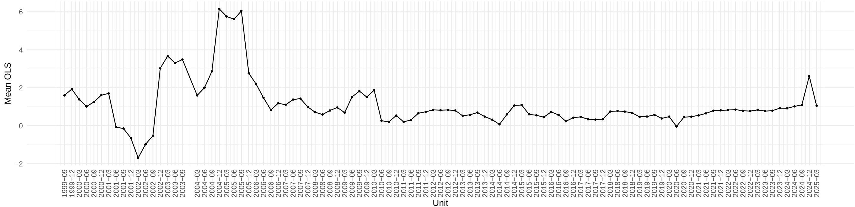
Evolution of INDPRO OLS coefficient across time
