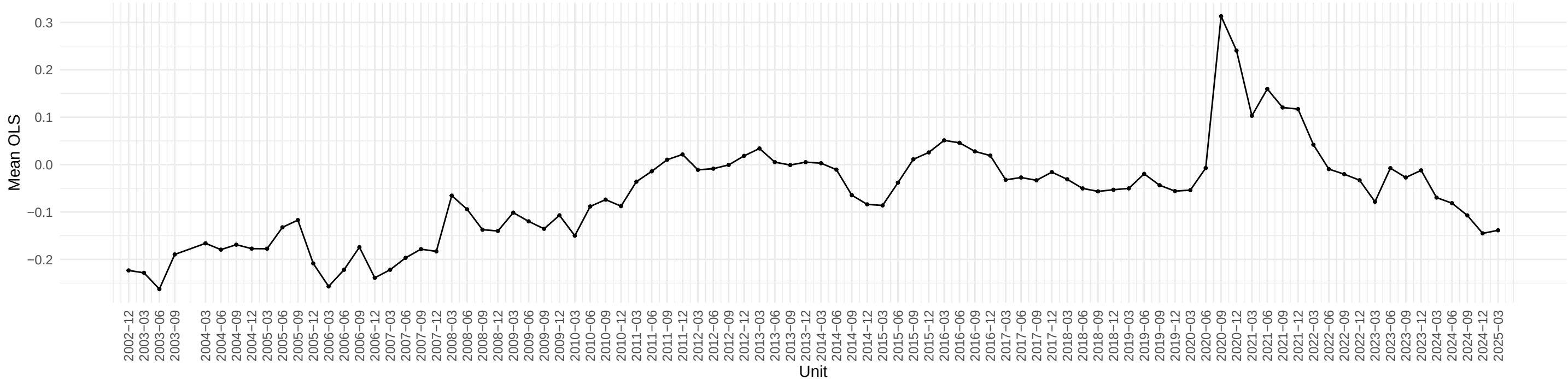
Evolution of IPBUSEQ OLS coefficient across time
