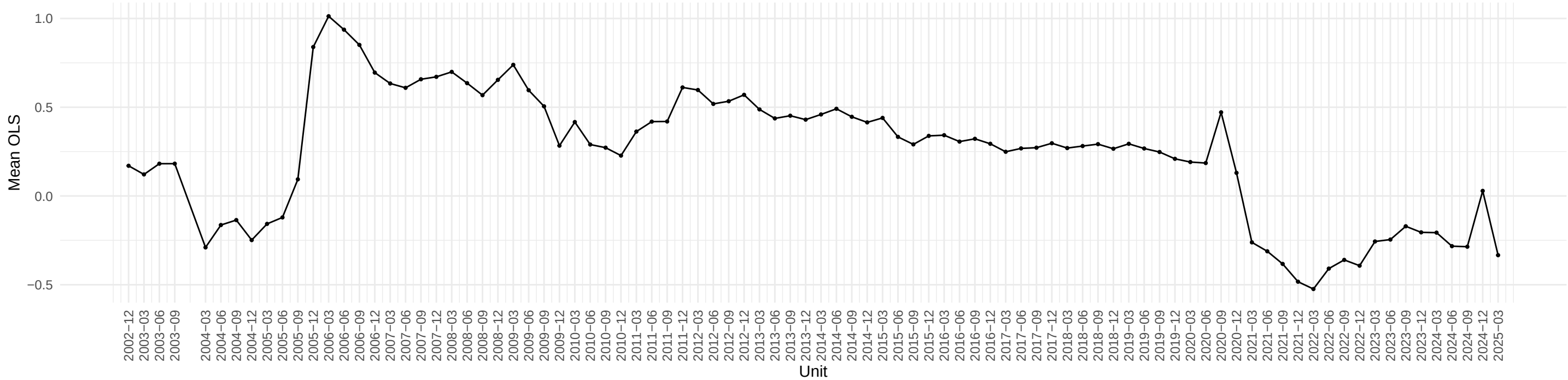
Evolution of IPDMAT OLS coefficient across time
