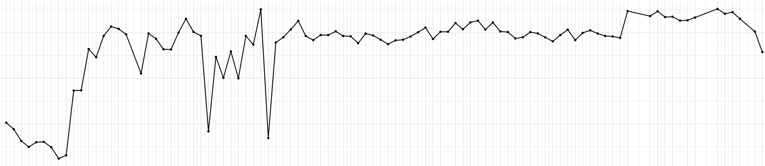
Evolution of M1SL OLS coefficient across time
