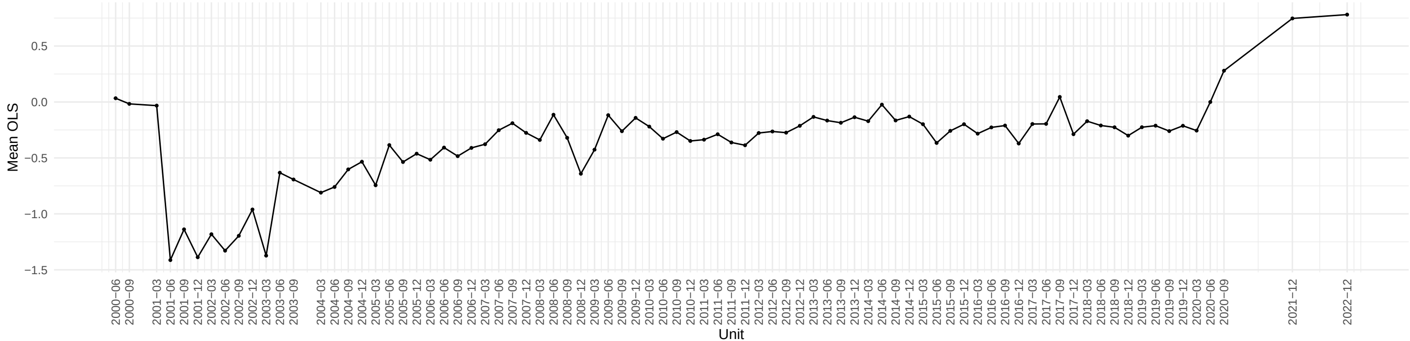
Evolution of OILPRICEx OLS coefficient across time
