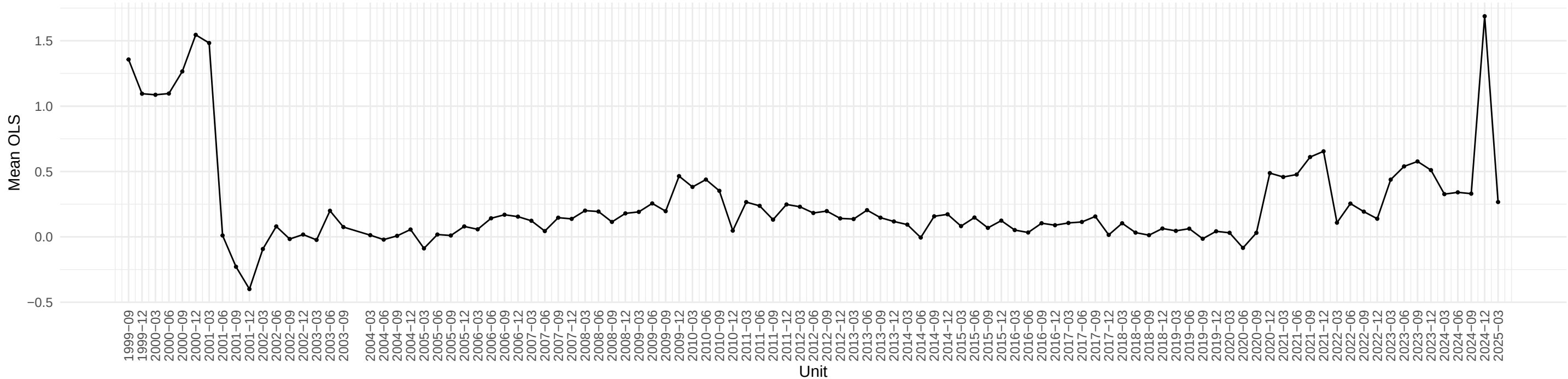
Evolution of PAYEMS OLS coefficient across time
