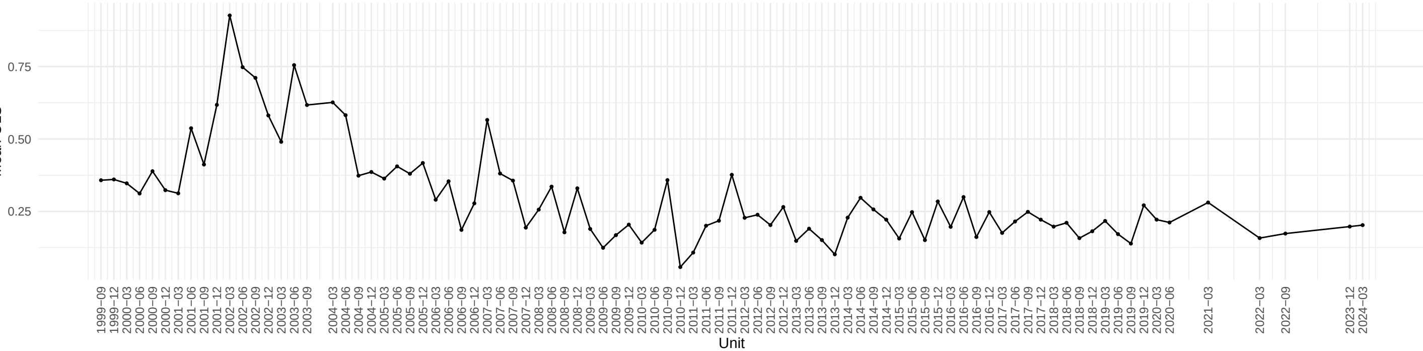
Evolution of PERMIT OLS coefficient across time
