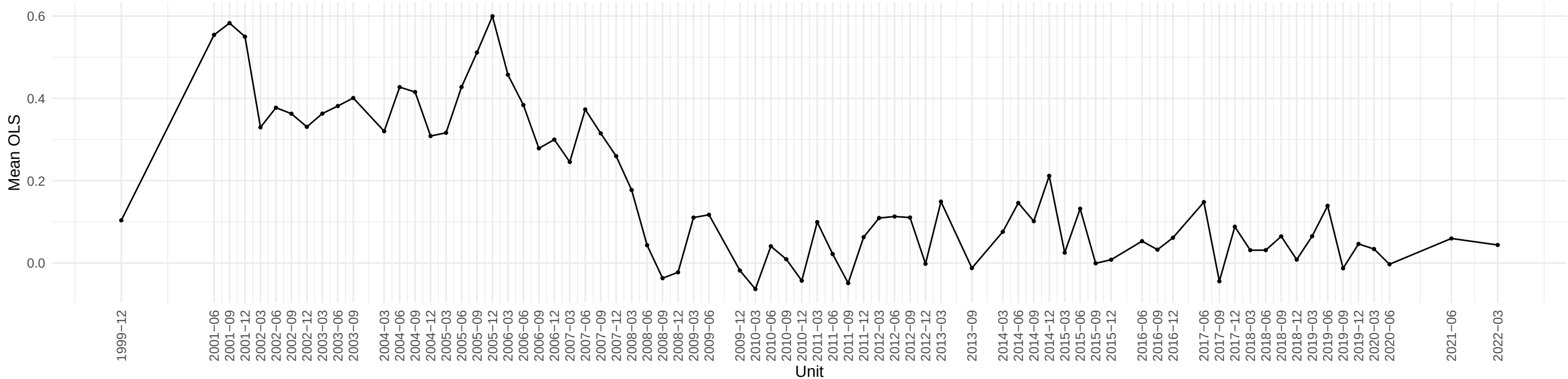
Evolution of PPICMM OLS coefficient across time
