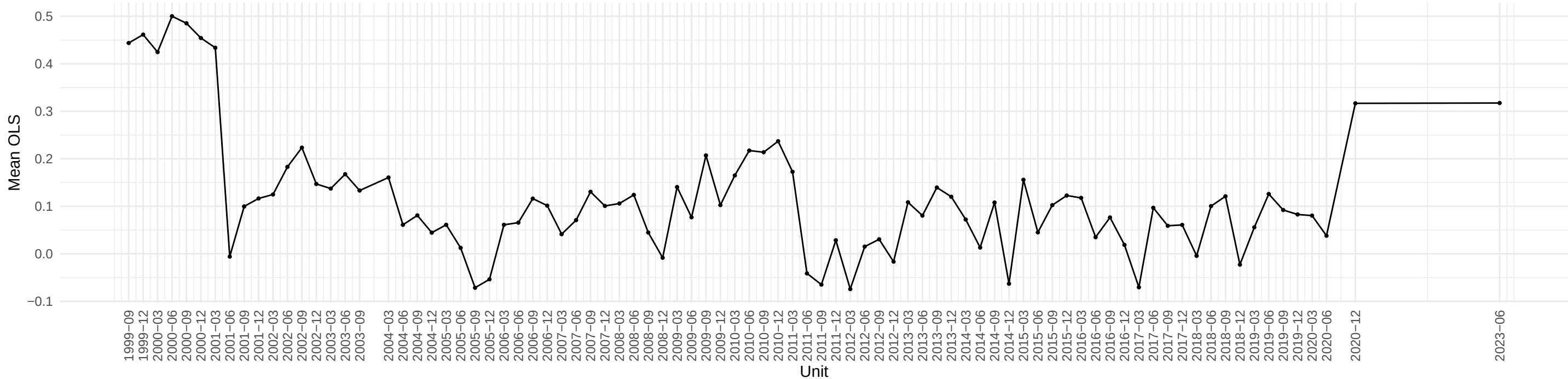
Evolution of RETAILx OLS coefficient across time
