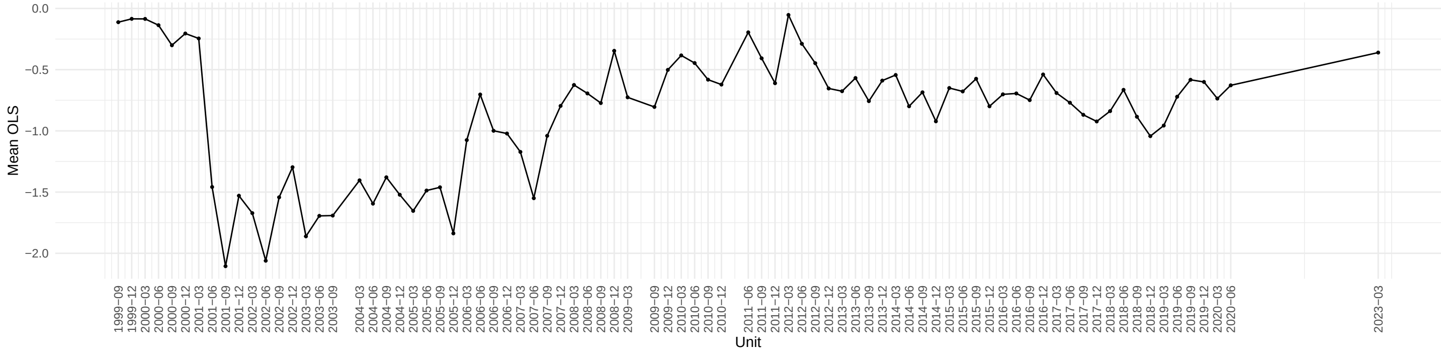
Evolution of TB3SMFFM OLS coefficient across time
