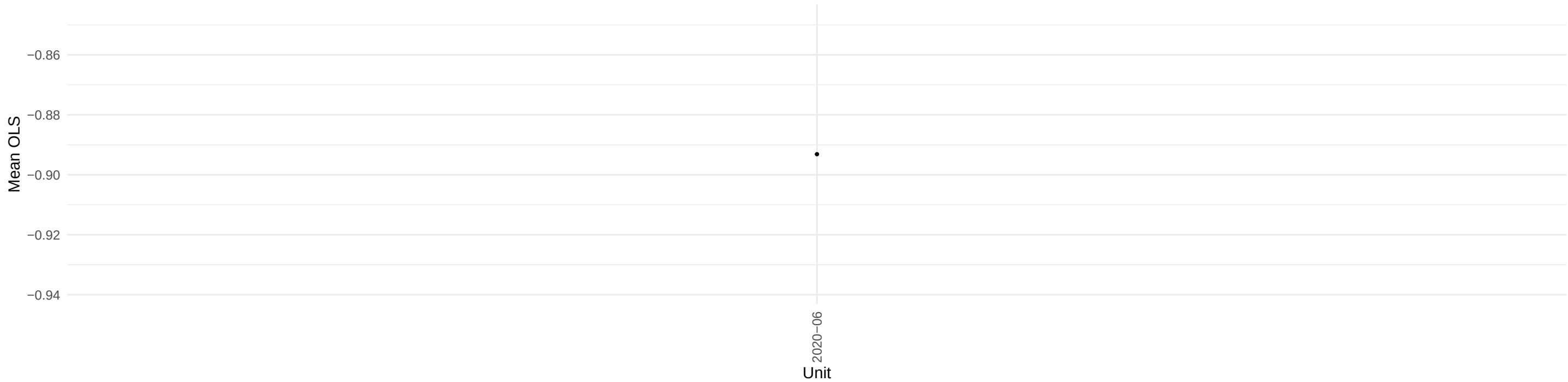
Evolution of TWEXAFEGSMTHx OLS coefficient across time
