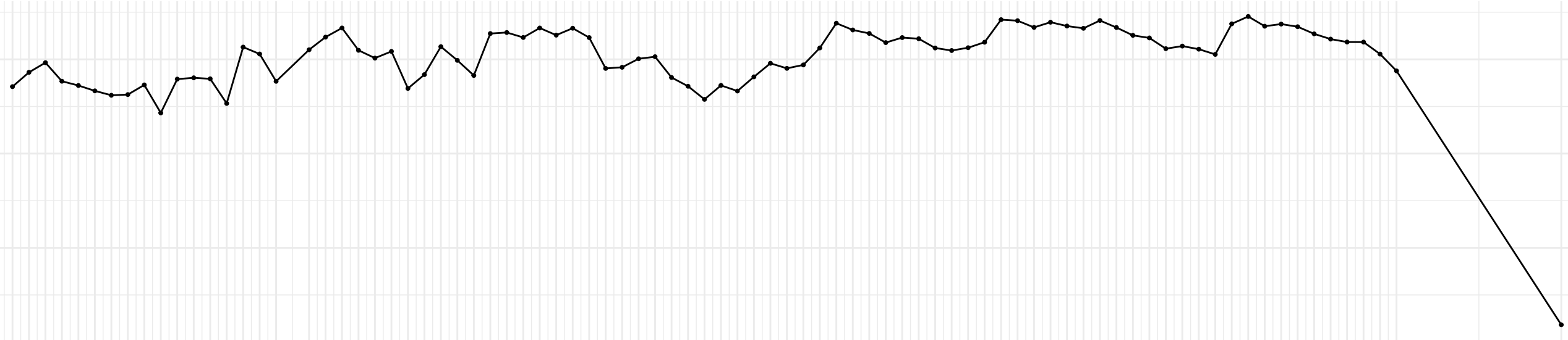
Evolution of UEMP15OV OLS coefficient across time
