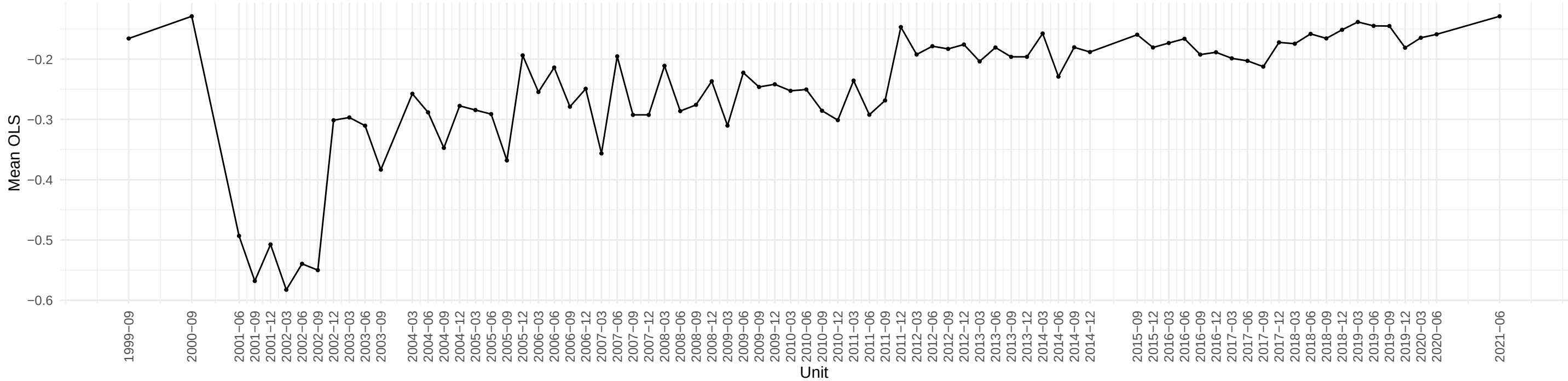
Evolution of VXOCLSx OLS coefficient across time
