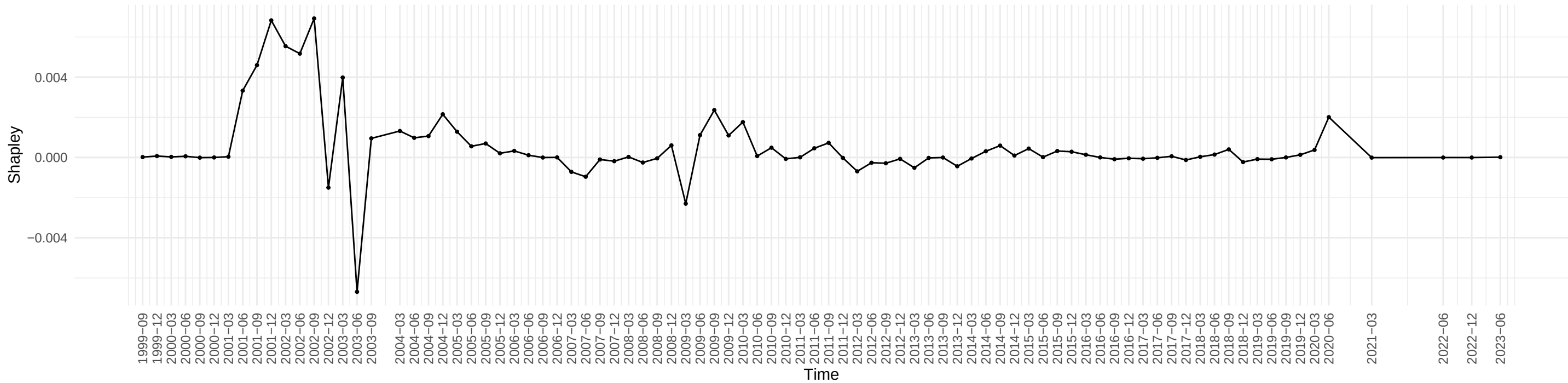
Evolution of Shapley Value of CES0600000007 across time
