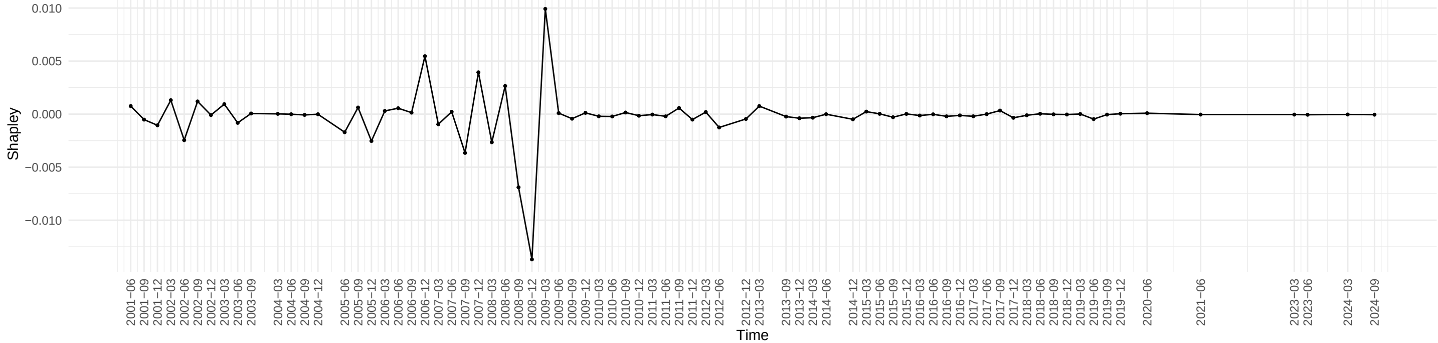
Evolution of Shapley Value of CPIAUCSL across time
