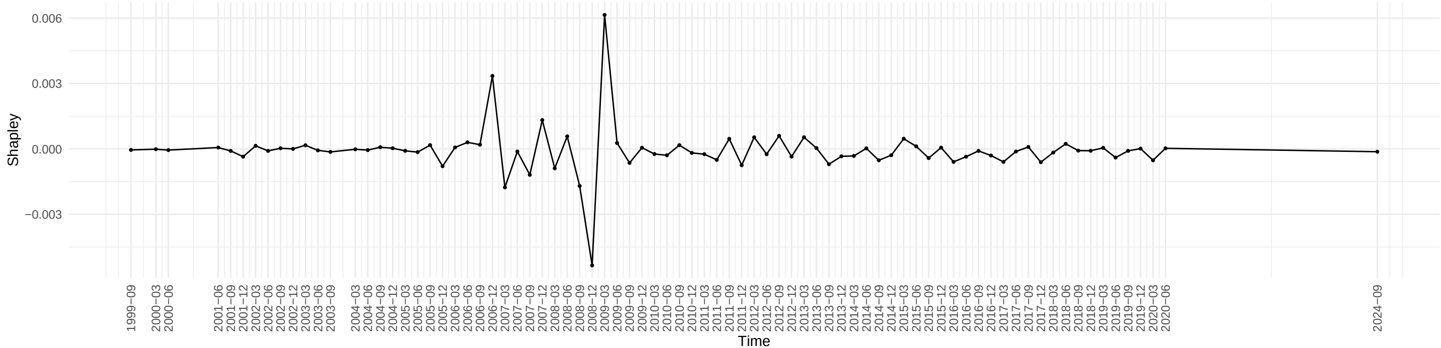
Evolution of Shapley Value of CPITRNSL across time
