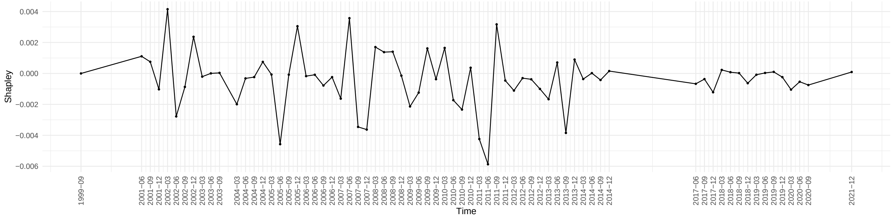
Evolution of Shapley Value of CUSR0000SAD across time
