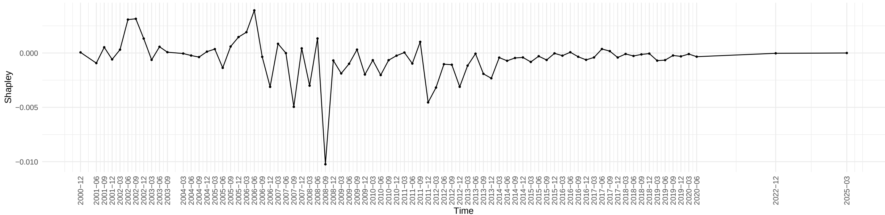
Evolution of Shapley Value of CUSR0000SAS across time
