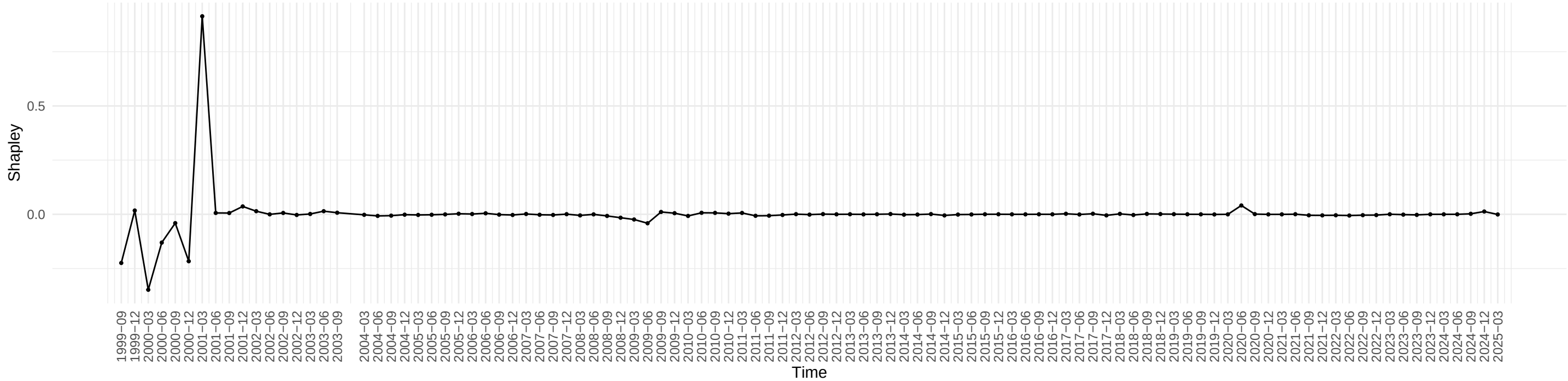
Evolution of Shapley Value of DMANEMP across time
