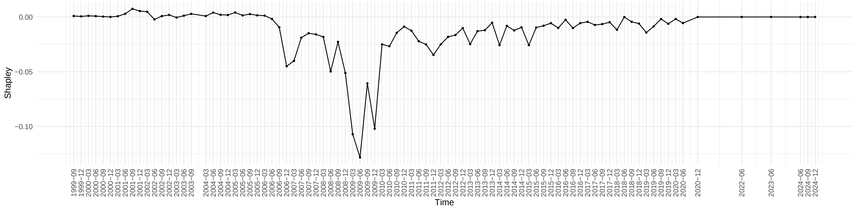
Evolution of Shapley Value of HOUSTMW across time
