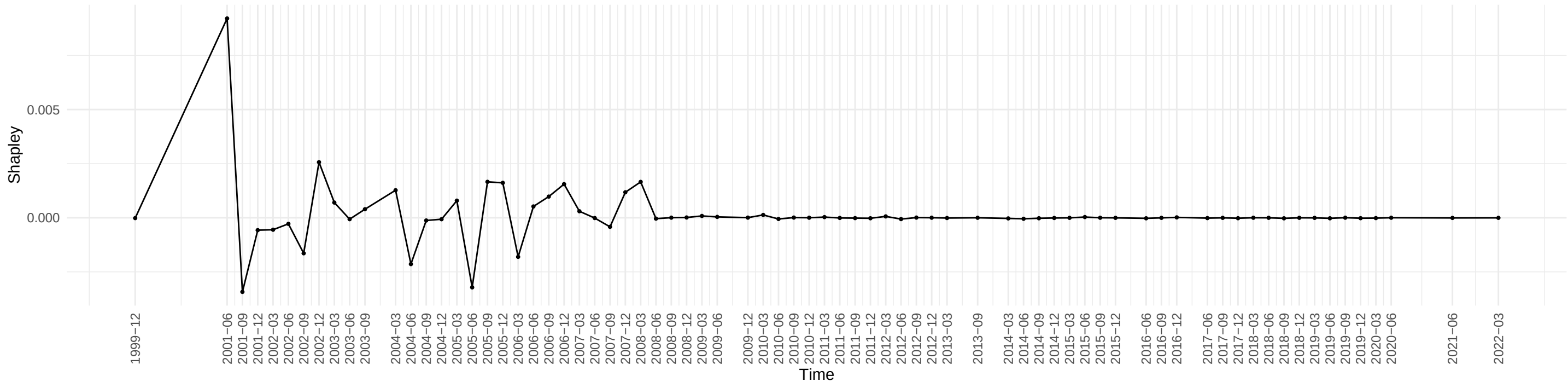
Evolution of Shapley Value of PPICMM across time
