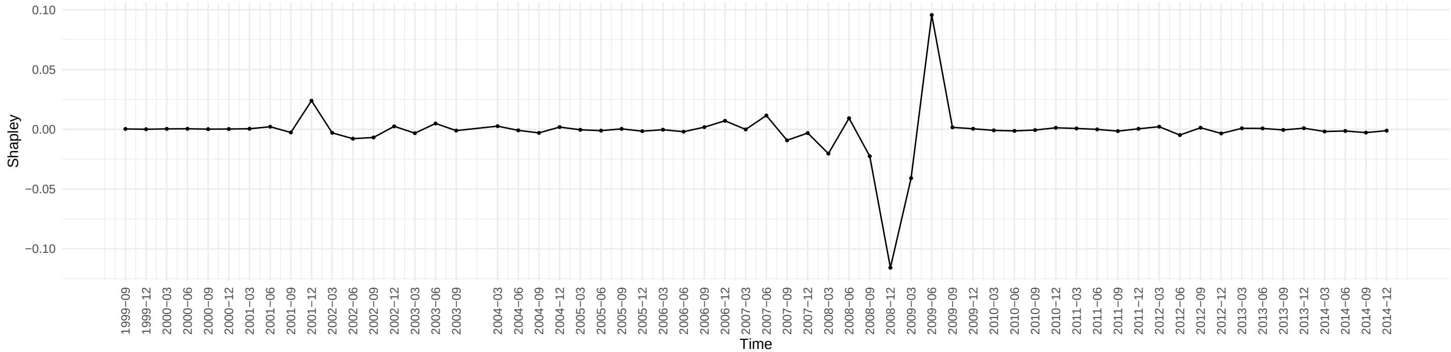
Evolution of Shapley Value of S&P: indust across time
