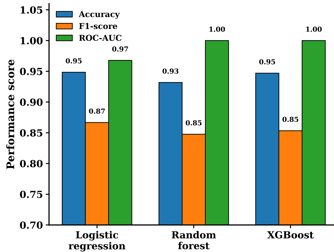
Model performance
