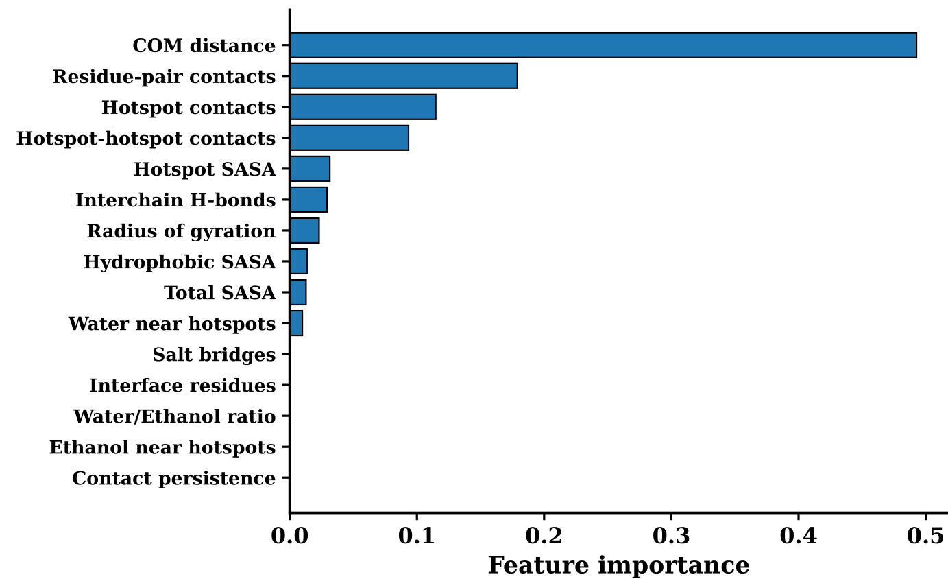
XGBoost
