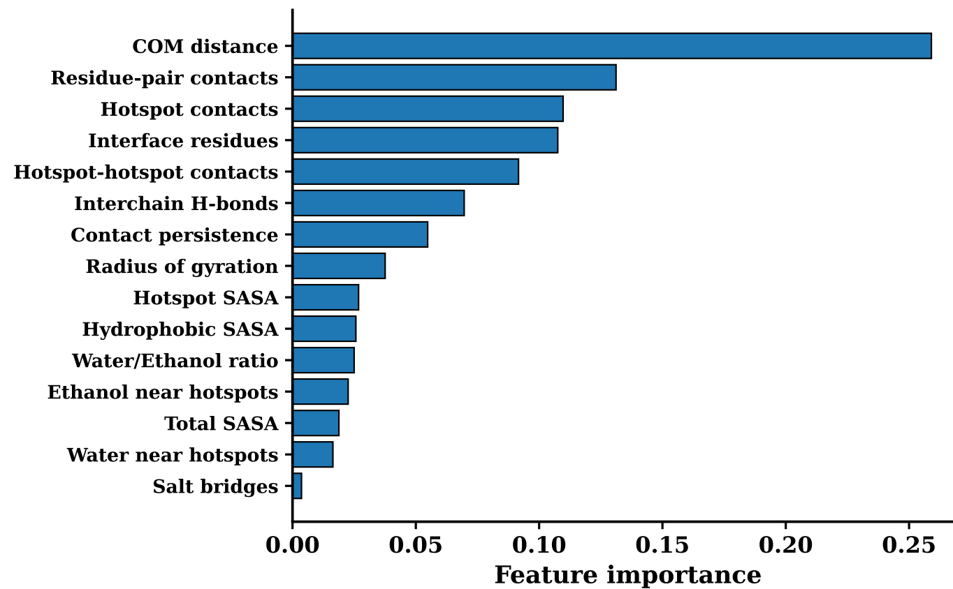
Random forest
