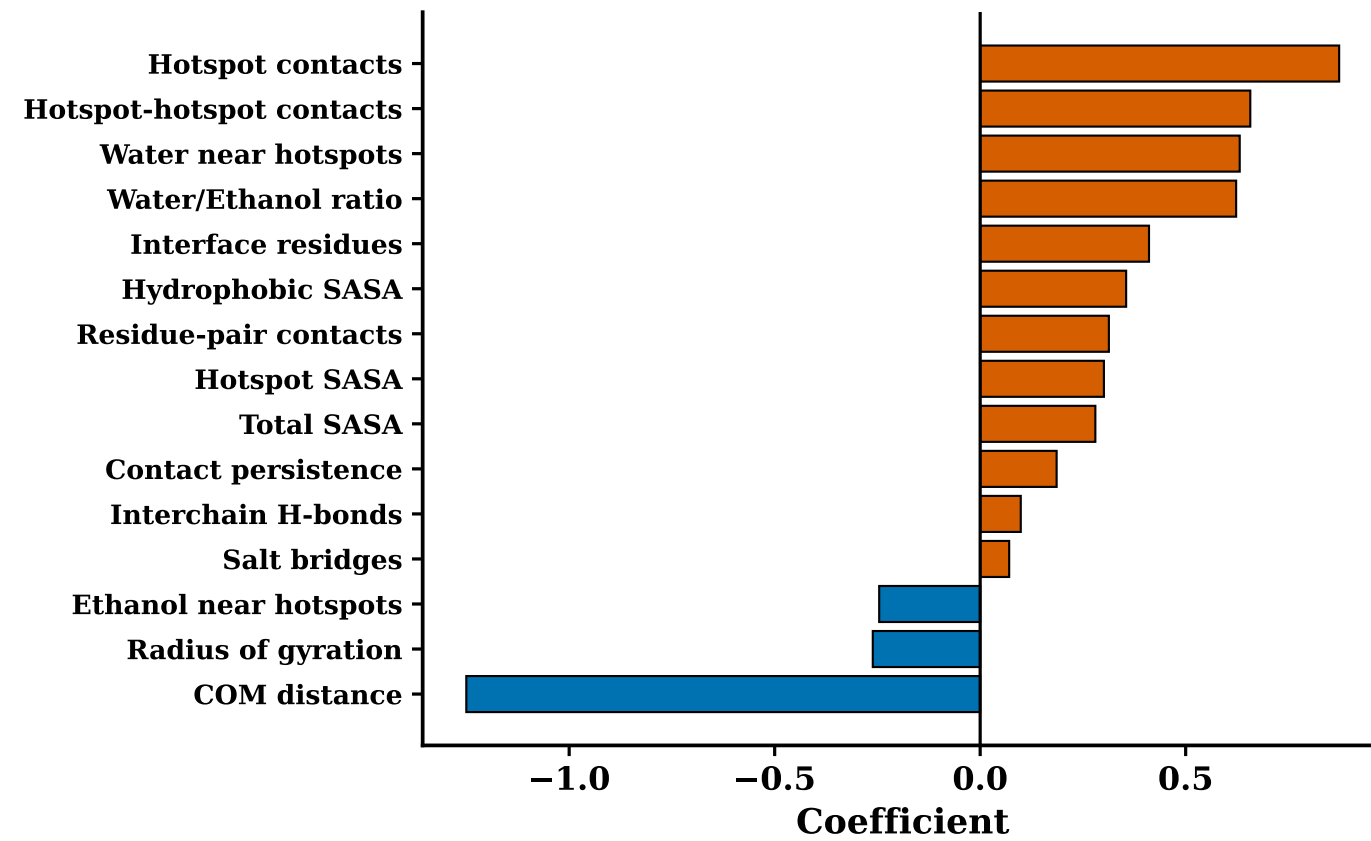
Logistic regression
