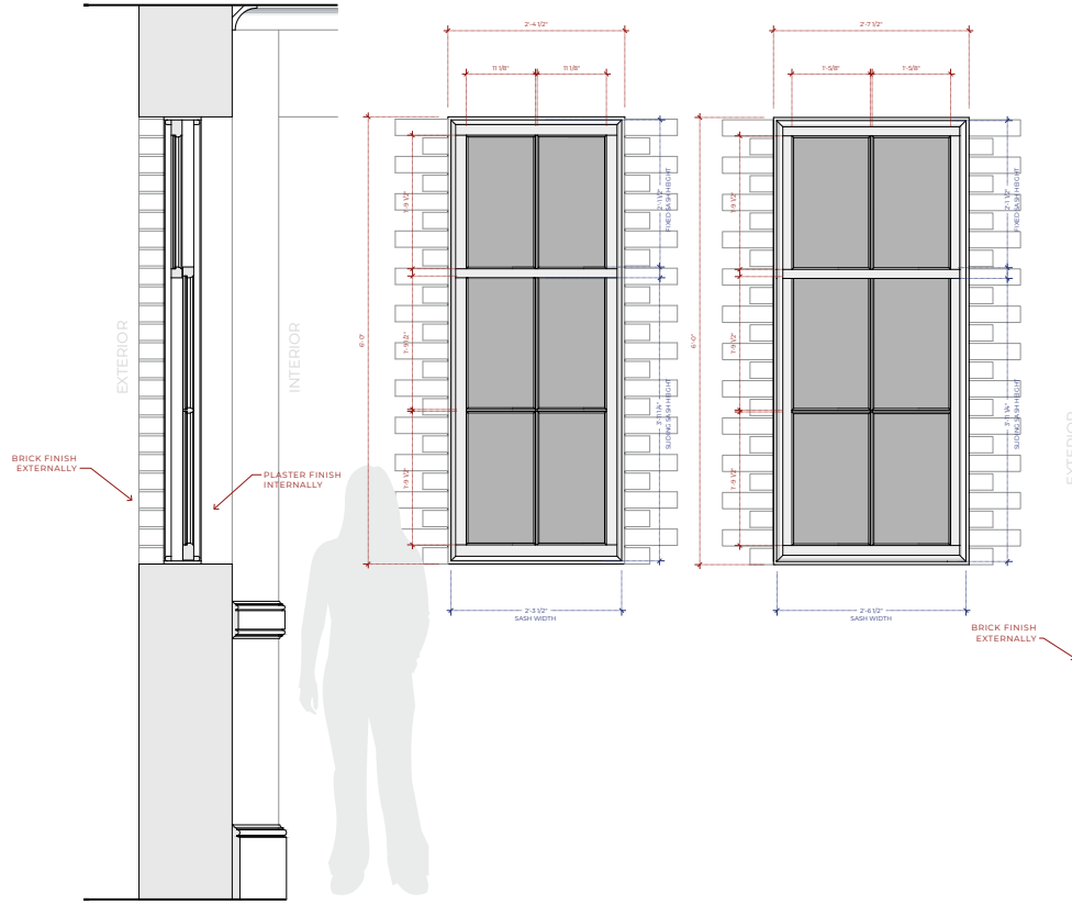
WINDOW TYPE 'A' LIGHTWELL WINDOWS 4x
