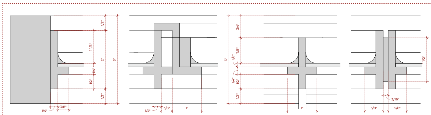
Detail 2 Scale: Full Scale
