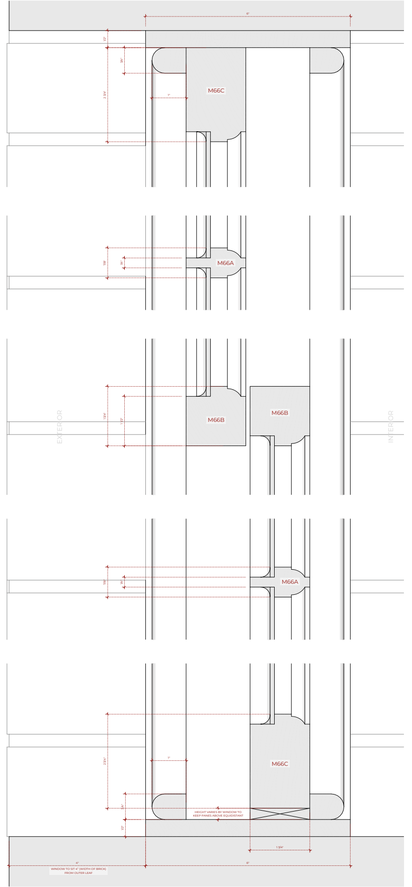
Typical Detail - Section Scale: Full Scale
