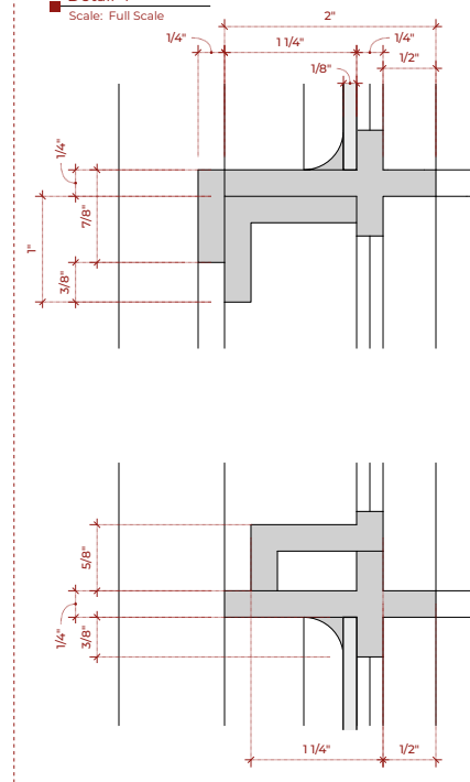
Detail 4 Scale: Full Scale
