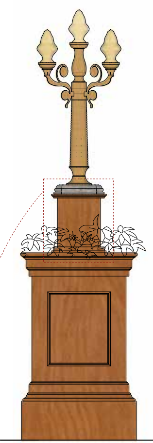
Typical Side Elevation For Type B & Type C Scale: 1" : 1'
