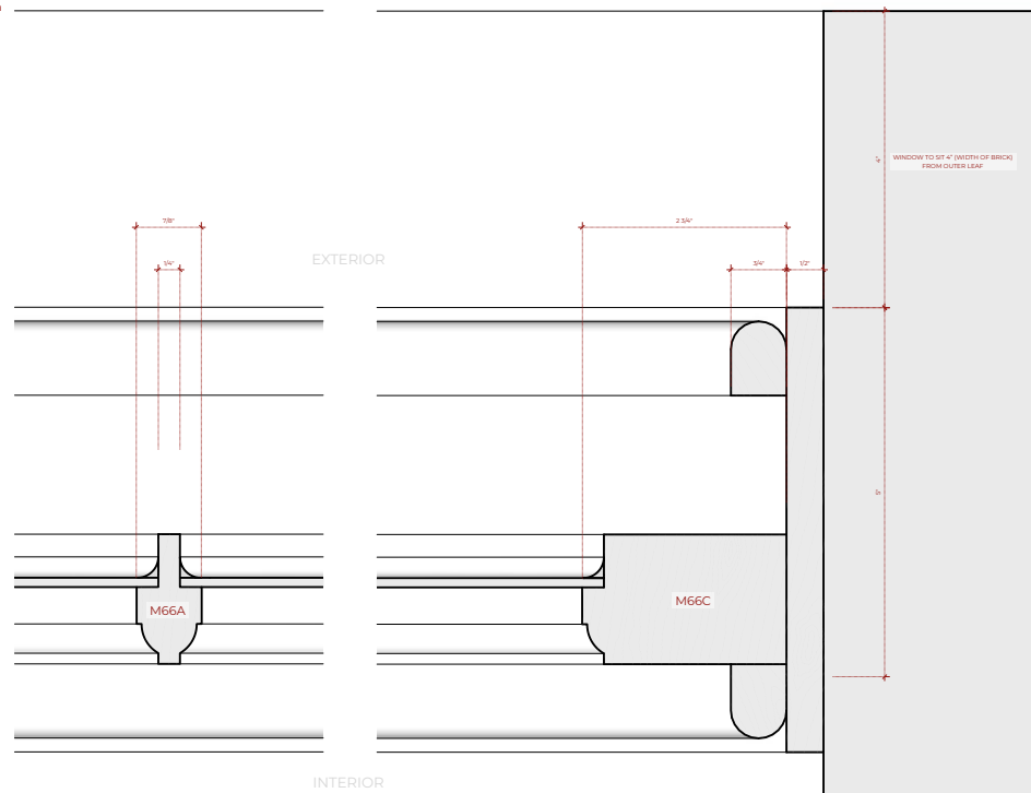
Typical Detail - Plan Scale: Full Scale
