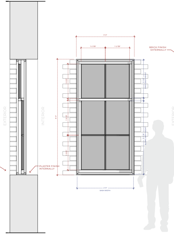
WINDOW TYPE 'C' STORE ROOM 1x
