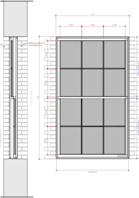
WINDOW TYPE 'D' BED ROOM 1x
