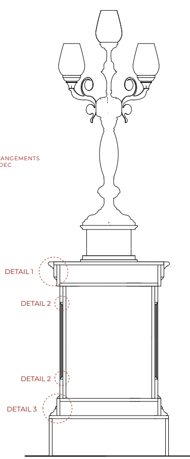
Typical Section For Type B & Type C Scale: 1" : 1'
