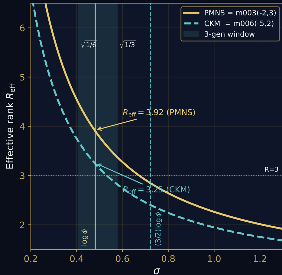
Geodesic length kernel: soft dimensional transition
