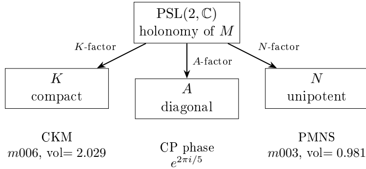
Figure 4: Iwasawa decomposition \text{PSL}(2, \mathbb{C}) = KAN of the holonomy representation of compact hyperbolic 3-manifolds with H_1 = \mathbb{Z}/5 . The K -factor (maximal compact) yields the CKM matrix from manifold m006 ; the N -factor (unipotent) yields the PMNS matrix from the Meyerhoff manifold m003 ; the A -factor (diagonal) encodes CP-violating twist angles quantized by the \mathbb{Z}/5 torsion.
