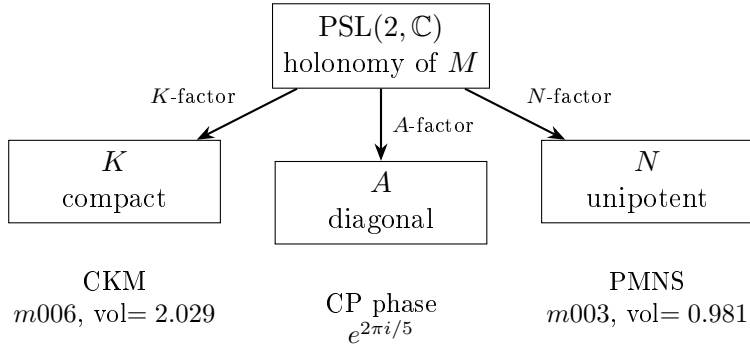
Figure 4: Iwasawa decomposition \mathrm{PSL}(2, \mathbb{C}) = KAN of the holonomy representation of compact hyperbolic 3-manifolds with H_1 = \mathbb{Z}/5 . The K -factor (maximal compact) yields the CKM matrix from manifold m006 ; the N -factor (unipotent) yields the PMNS matrix from the Meyerhoff manifold m003 ; the A -factor (diagonal) encodes CP-violating twist angles quantized by the \mathbb{Z}/5 torsion.
