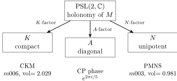
Figure 4: Iwasawa decomposition \mathrm{PSL}(2, \mathbb{C}) = KAN of the holonomy representation of compact hyperbolic 3-manifolds with H_1 = \mathbb{Z}/5 . The K -factor (maximal compact) yields the CKM matrix from manifold m006 ; the N -factor (unipotent) yields the PMNS matrix from the Meyerhoff manifold m003 ; the A -factor (diagonal) encodes CP-violating twist angles quantized by the \mathbb{Z}/5 torsion.
