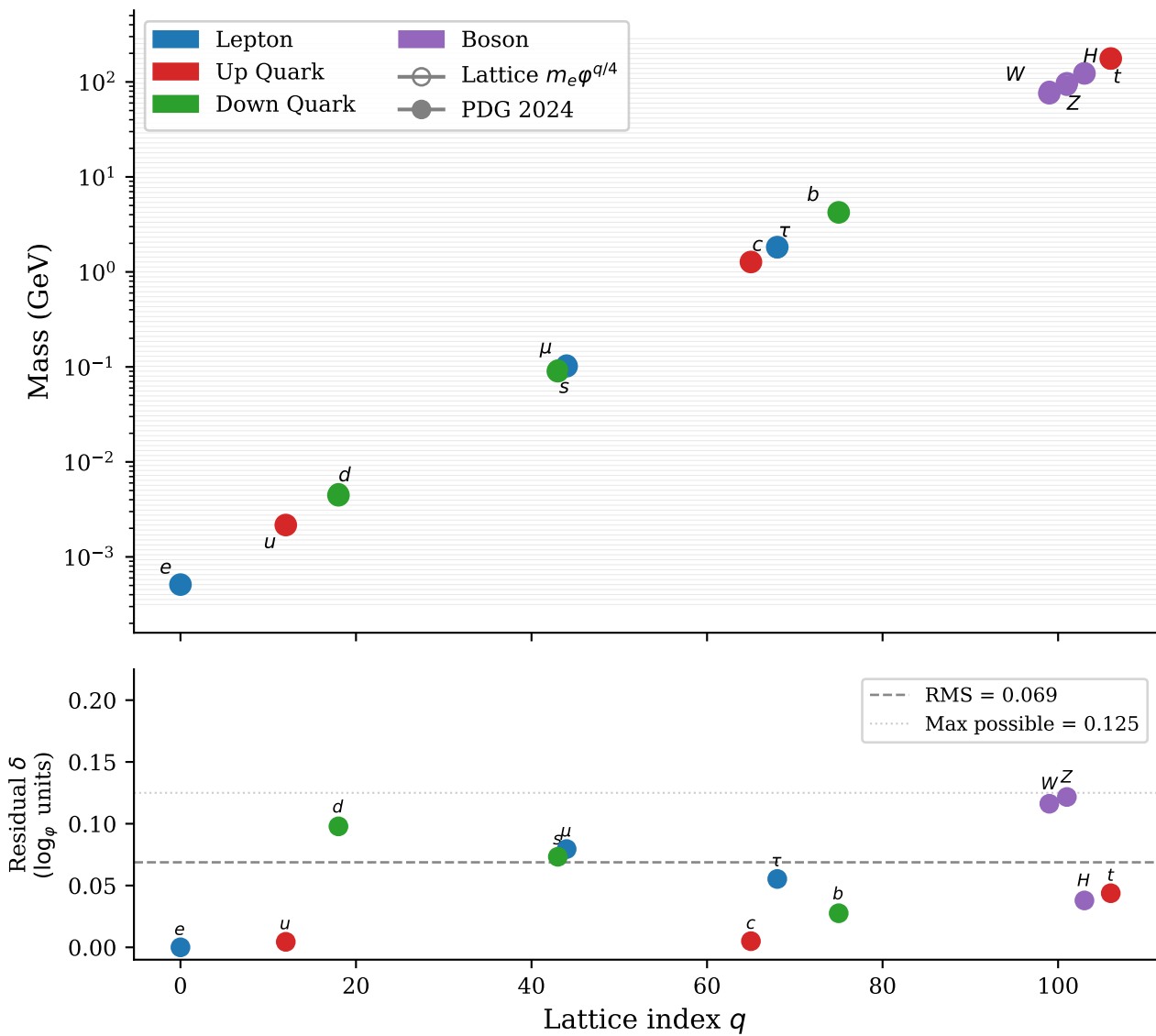
Standard Model masses on the \phi -lattice m = m_e \phi^{q/4}
