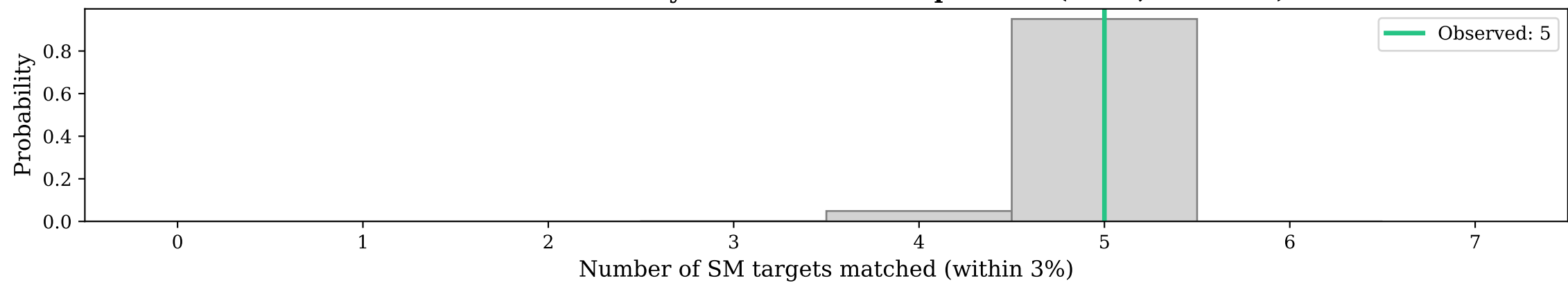
Null model: matches by uniform random spectrum (n=10,000 trials)
