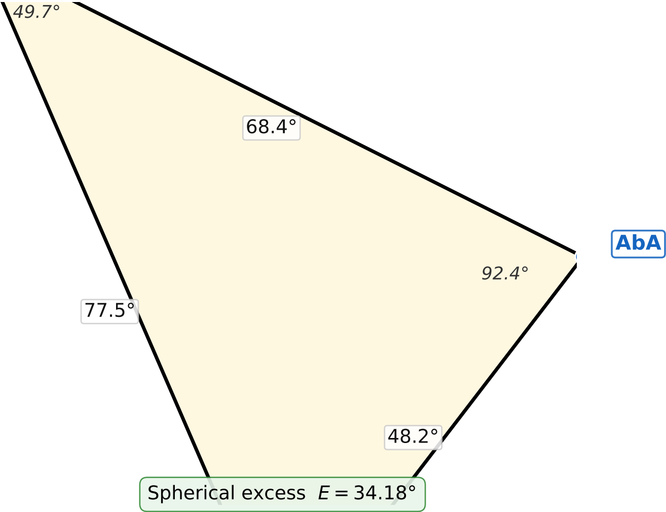
(b) Spherical triangle
