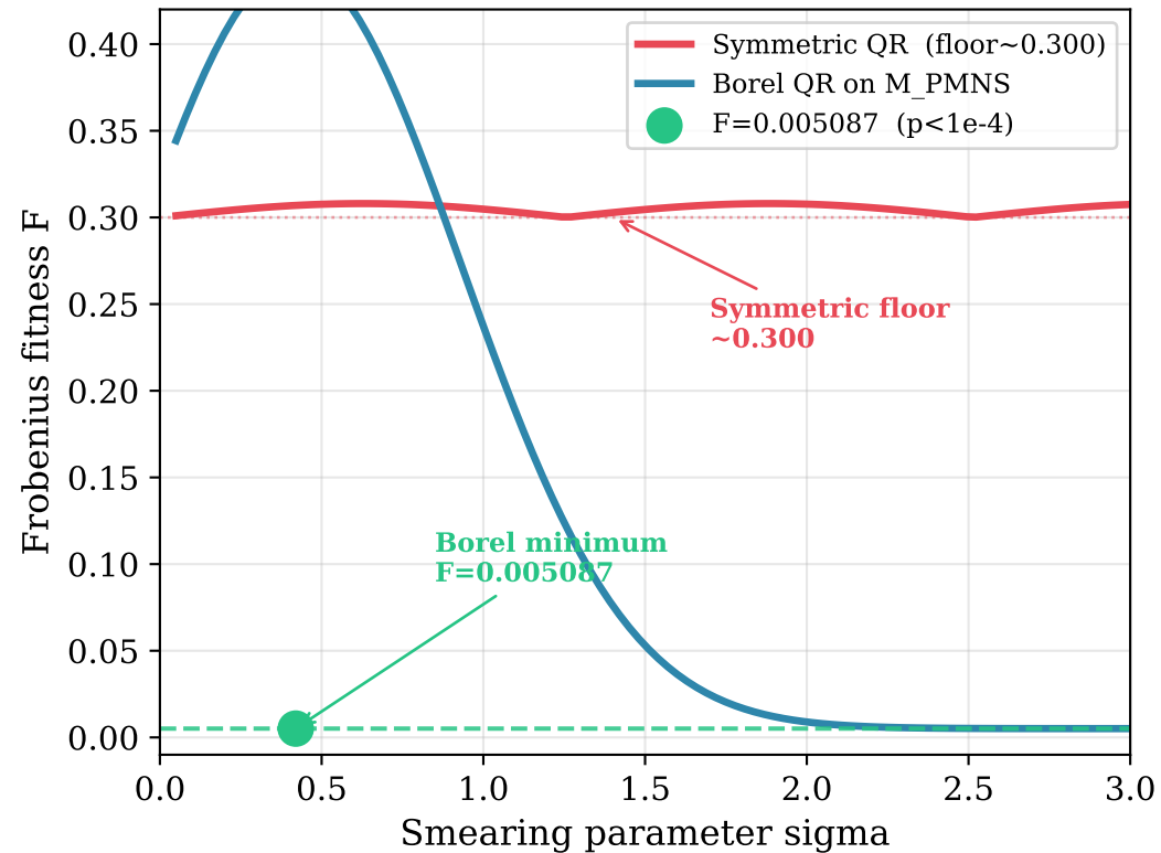
Symmetric QR obstruction vs Borel construction
