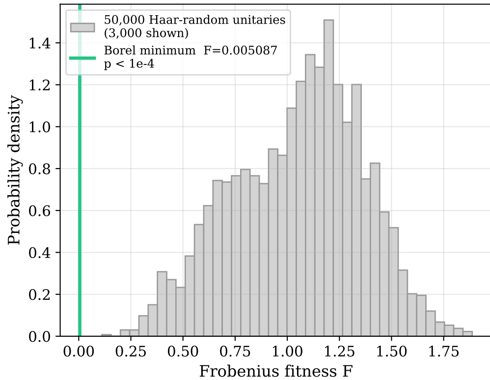
Statistical significance vs Haar-random unitaries
