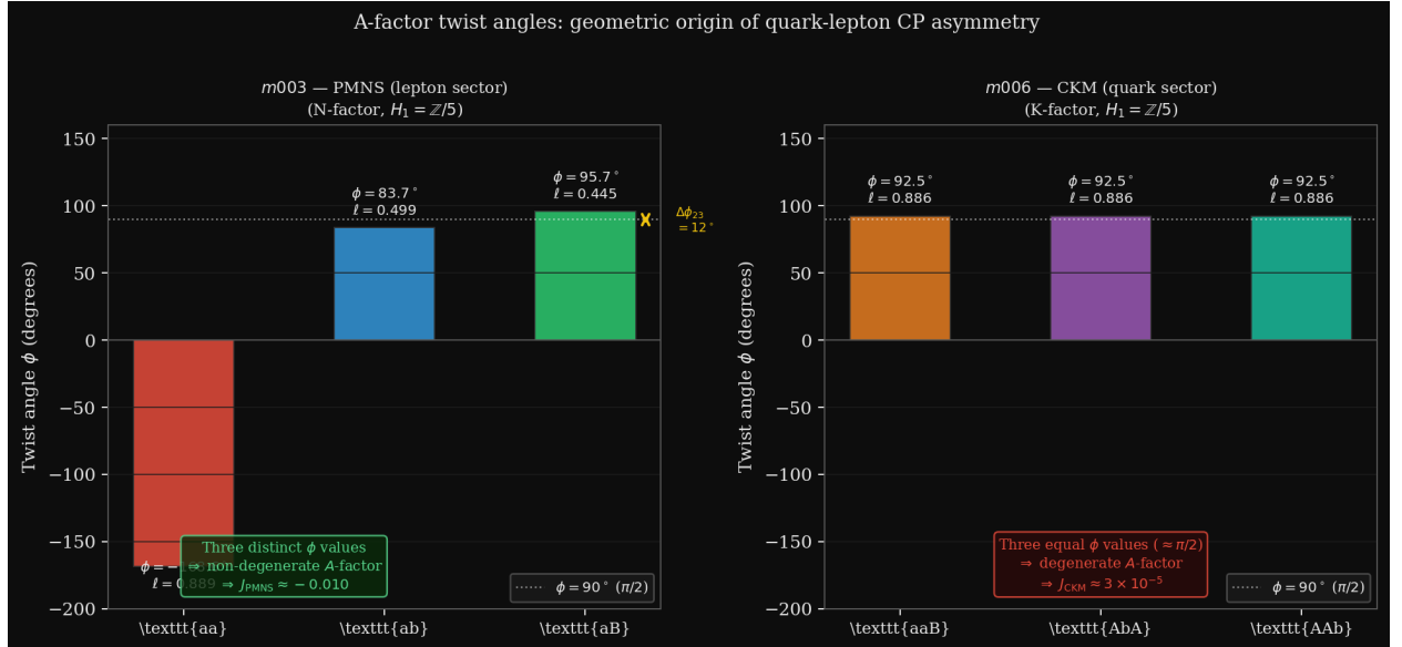
FIG. 2. A-factor twist angles \phi(\gamma) for the optimal word triples on m003 (PMNS, left) and m006 (CKM, right). On m003 , the three words aa, ab, aB have three distinct twist angles (-168.6^\circ, 83.7^\circ, 95.7^\circ) , producing a non-degenerate A -factor and J_{\text{PMNS}} \approx -0.010 . On m006 , all three words aaB, AbA, AAb share the same twist angle \phi \approx 92.5^\circ \approx \pi/2 , producing a degenerate A -factor and the observed suppression J_{\text{CKM}} \approx 3 \times 10^{-5} \ll J_{\text{PMNS}} . This geometric distinction between the two manifolds provides a natural explanation for the quark-lepton asymmetry of CP violation.
