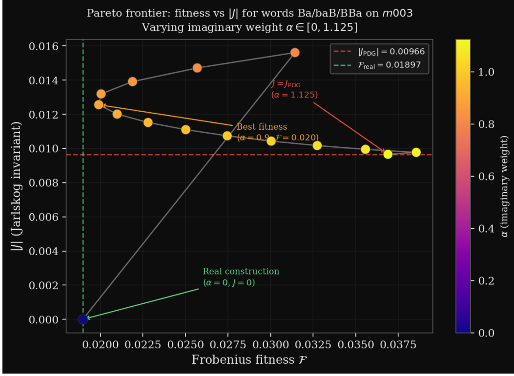
FIG. 1. Pareto frontier in the (\mathcal{F}, |J|) plane for the complex Borel construction on m003 with word triple Ba/baB/BBa, as the imaginary weight \alpha varies from 0 to 1.125. The real construction ( \alpha = 0 , green dashed line) achieves \mathcal{F} = 0.019 with J = 0 . Increasing \alpha continuously trades fitness for CP phase: at \alpha = 0.9 the fitness remains 0.020 while |J| = 0.013 ; at \alpha = 1.125 the Jarlskog invariant matches the PDG value |J_{\text{PDG}}| = 0.00966 (red dashed line) exactly. Color encodes \alpha . Values \alpha > 1 are geometrically permitted since the norm in (8) is well-defined for all \alpha \geq 0 .
