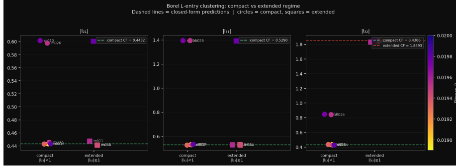
Fig. 2 Clustering of optimal Borel L -entries across the census scan, separated by regime ( |l_{32}| < 1 : compact, circles; |l_{32}| \geq 1 : extended, squares). Color encodes fitness \mathcal{F} . Dashed lines show the closed-form predictions of Table 3: the compact and extended values of |l_{32}| are the two roots of the quadratic in Proposition 2. The entries |l_{21}| and |l_{31}| are universal across both regimes.
