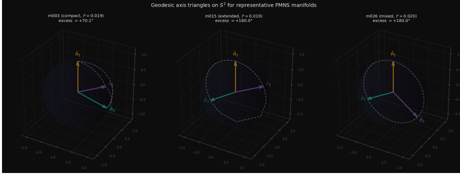
Fig. 1 Geodesic axis triangles on S^2 for three representative manifolds. Colored arrows show the three holonomy axis directions \hat{n}_1, \hat{n}_2, \hat{n}_3 ; dashed arcs are the geodesic edges of the spherical triangle. Left: m003 (compact regime, \mathcal{F} = 0.019 ); centre: m015 (extended regime, \mathcal{F} = 0.019 ); right: m026 ( H_1 = \mathbb{Z}/13 , \mathcal{F} = 0.020 ).
