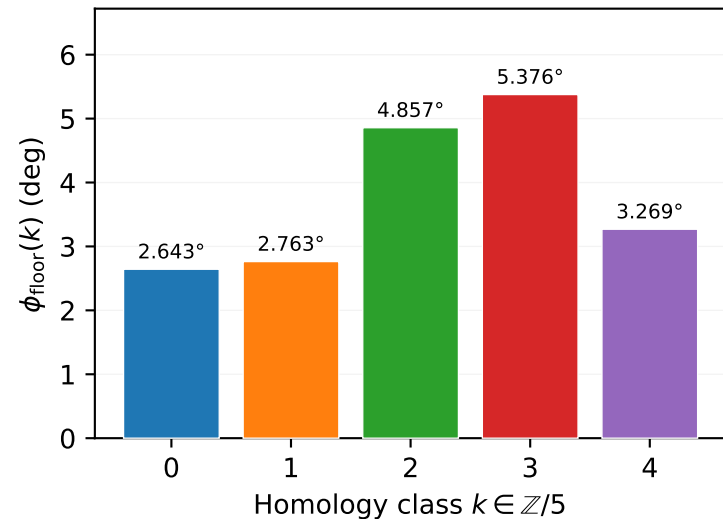
\texttt{m003} (Meyerhoff)
