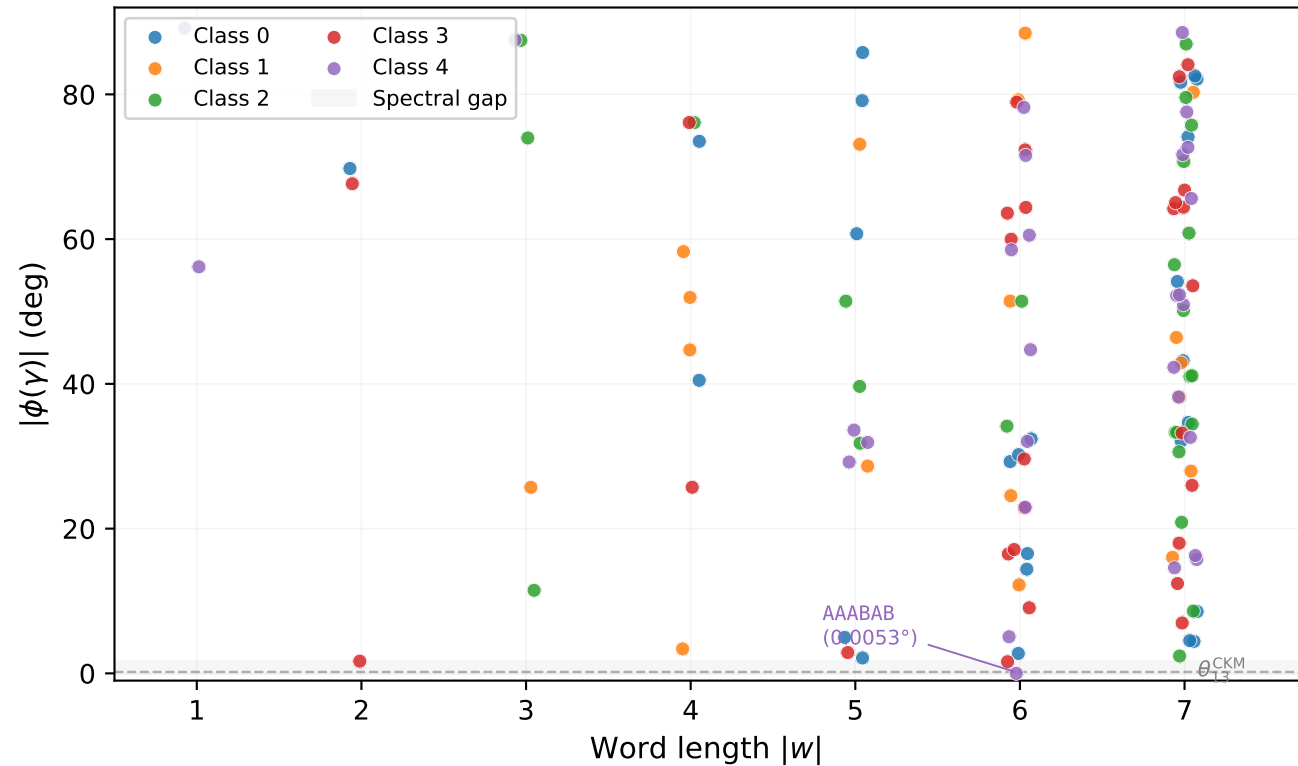
\texttt{m006}: twist spectrum by homology class
