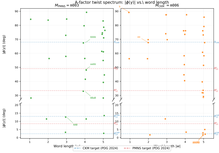
Fig. 1 A-factor twist spectrum |\phi(\gamma)| (folded to [0^\circ, 90^\circ] ) versus word length for m003 (left, green) and m006 (right, orange). Top panel: 27^\circ – 90^\circ . Bottom panel: 0^\circ – 21^\circ . Dashed lines: CKM targets (blue) and PMNS targets (red). The spectral gap between 21^\circ and 27^\circ is a genuine geometric feature of both manifolds. Annotated points mark the key coincidences per manifold.
