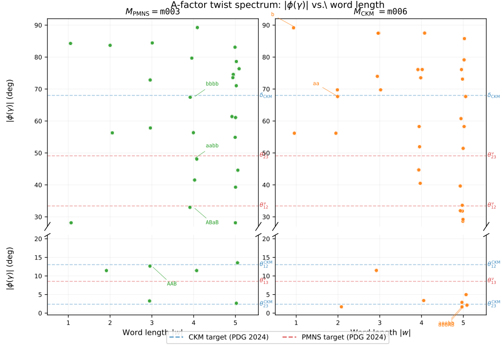
Figure 1: A-factor twist spectrum |\phi(\gamma)| (folded to [0^\circ, 90^\circ] ) versus word length for m003 (left, green) and m006 (right, orange). Top panel: 27^\circ – 90^\circ . Bottom panel: 0^\circ – 21^\circ . Dashed lines: CKM targets (blue) and PMNS targets (red). The spectral gap between 21^\circ and 27^\circ is a genuine geometric feature of both manifolds. Annotated points mark the key coincidences per manifold.
