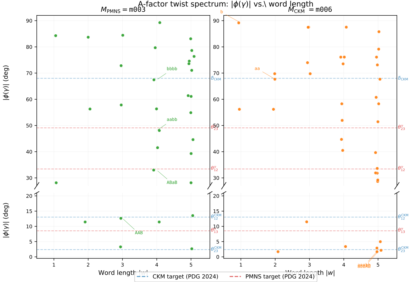
FIG. 1. A-factor twist spectrum |\phi(\gamma)| (folded to [0^\circ, 90^\circ] ) versus word length for m003 (left, green) and m006 (right, orange). Top panel: 27^\circ – 90^\circ . Bottom panel: 0^\circ – 21^\circ . Dashed lines: CKM targets (blue) and PMNS targets (red). The spectral gap between 21^\circ and 27^\circ is a genuine geometric feature of both manifolds. Annotated points mark the key coincidences per manifold.
