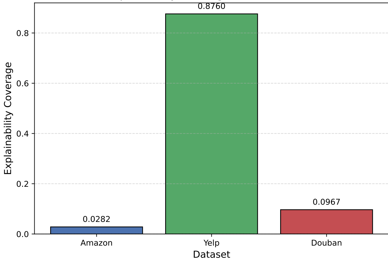
Explainability Coverage Across Datasets
