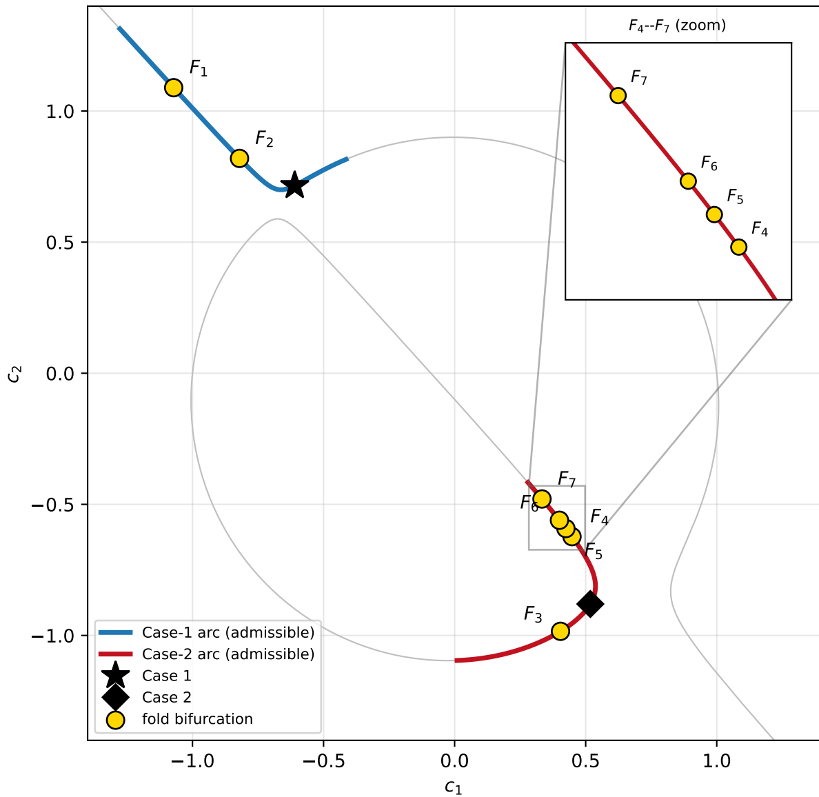
Admissible CC arcs (grey: full \psi = 0 level set)
