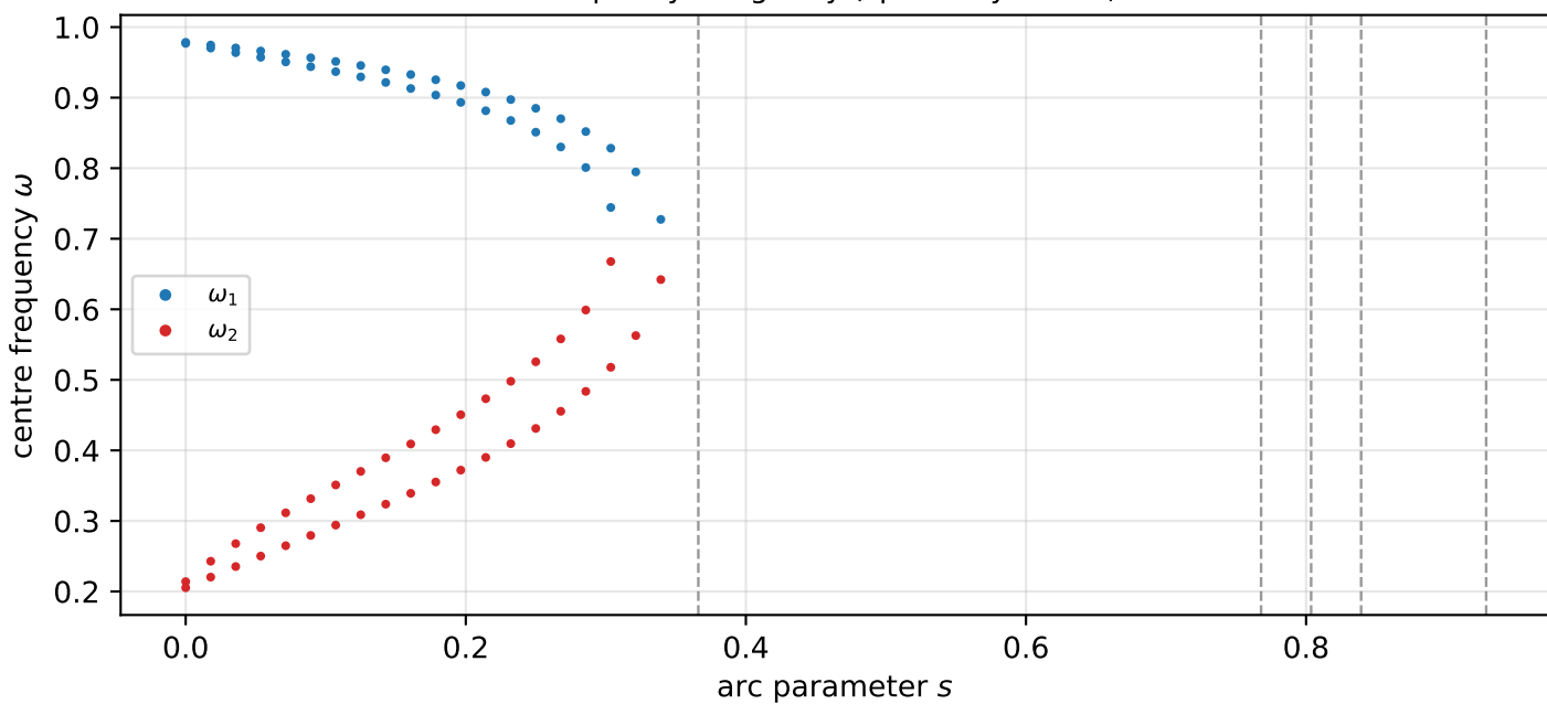
Case-2 arc: purely-imaginary (spectrally stable) intervals
