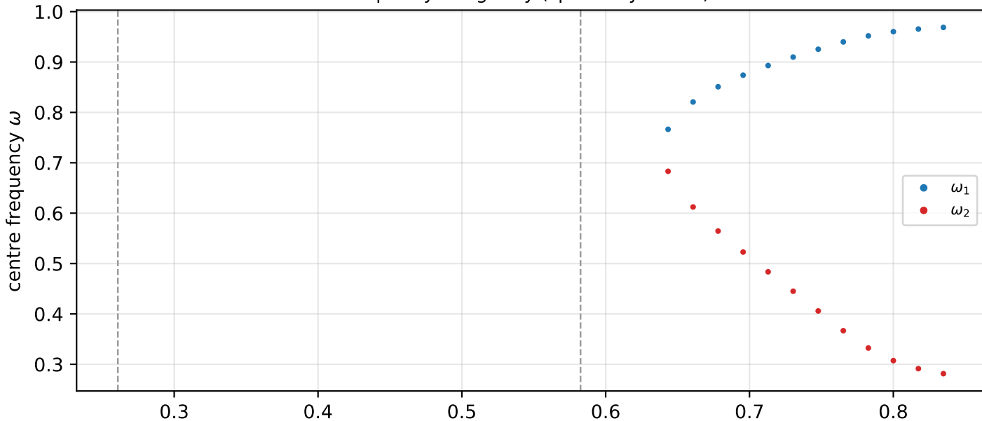
Case-2 arc: purely-imaginary (spectrally stable) intervals
