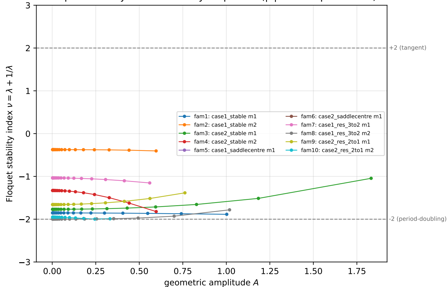
Floquet stability index vs family amplitude ( |\nu| < 2 : Floquet stable)
