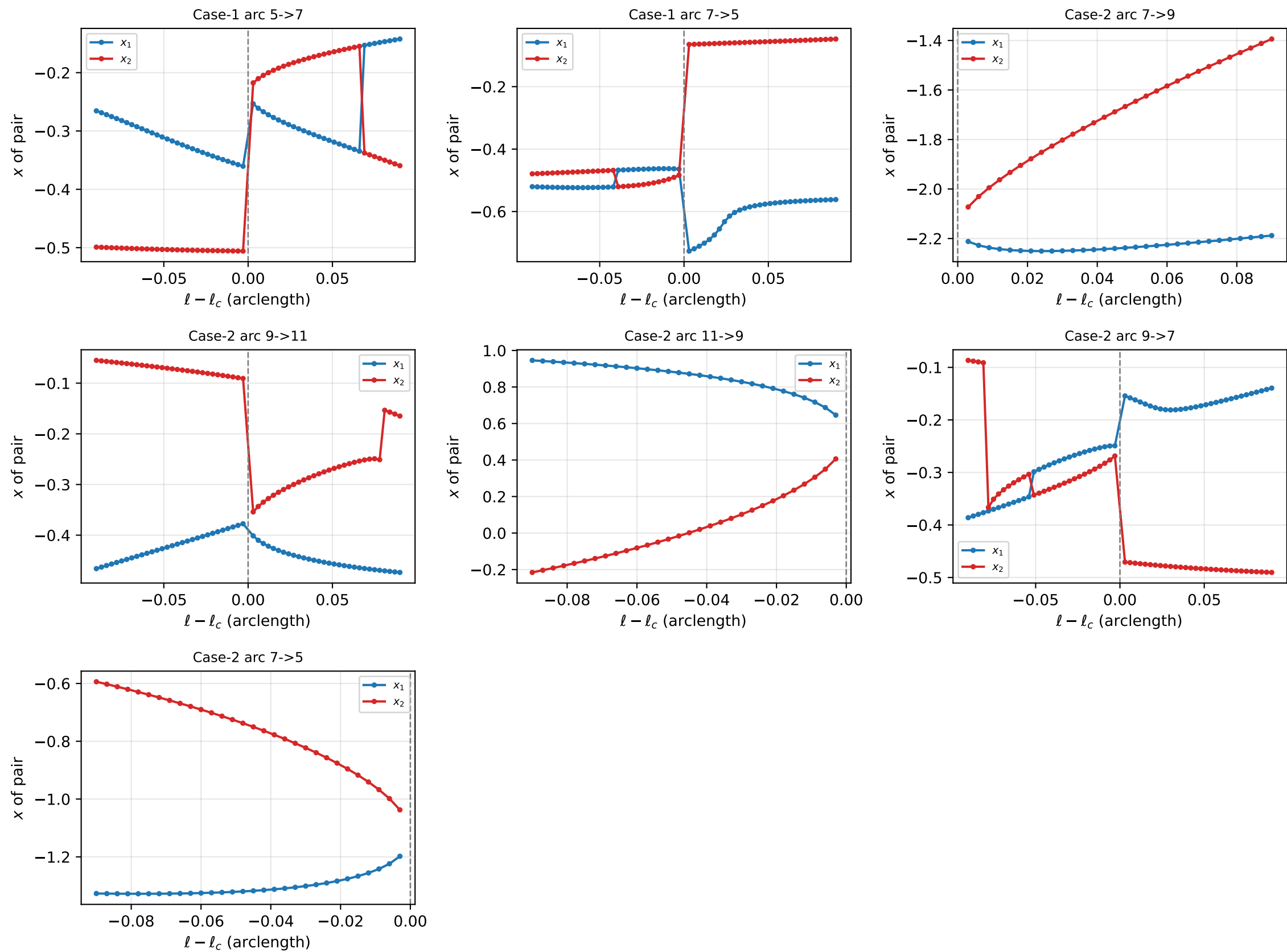
Local branch structure at each saddle-node (merging pair coordinates; fold at \ell = \ell_c )
