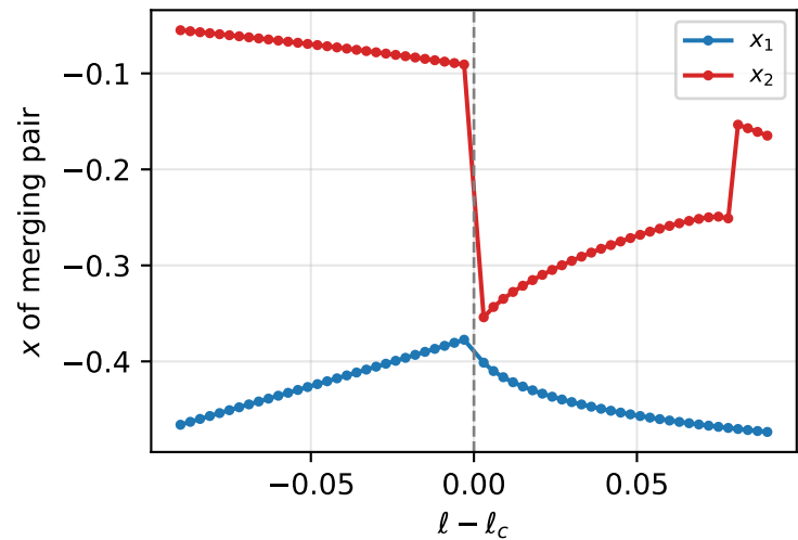
N = 11 -bounding fold ( 9 \rightarrow 11 )
