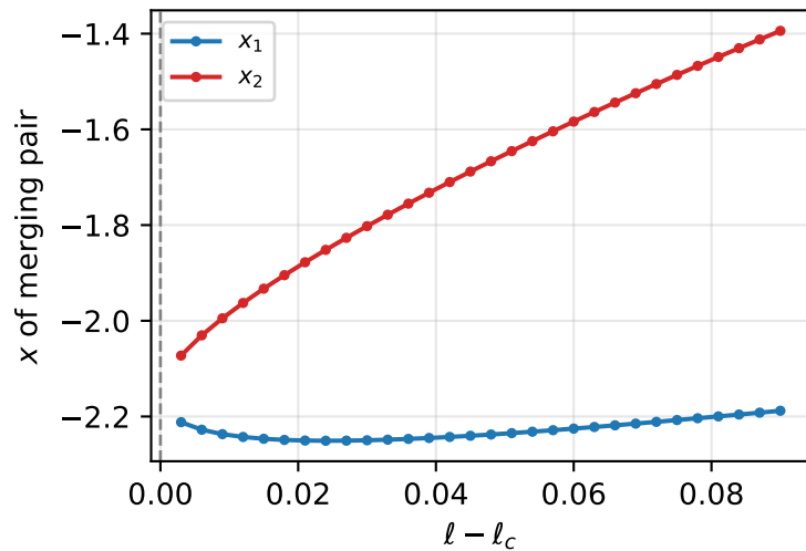
Case-2 fold ( 7 \rightarrow 9 )
