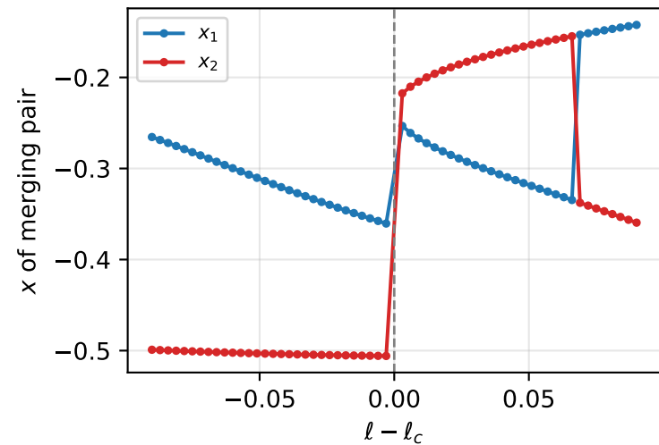
Case-1 fold ( 5 \rightarrow 7 )
