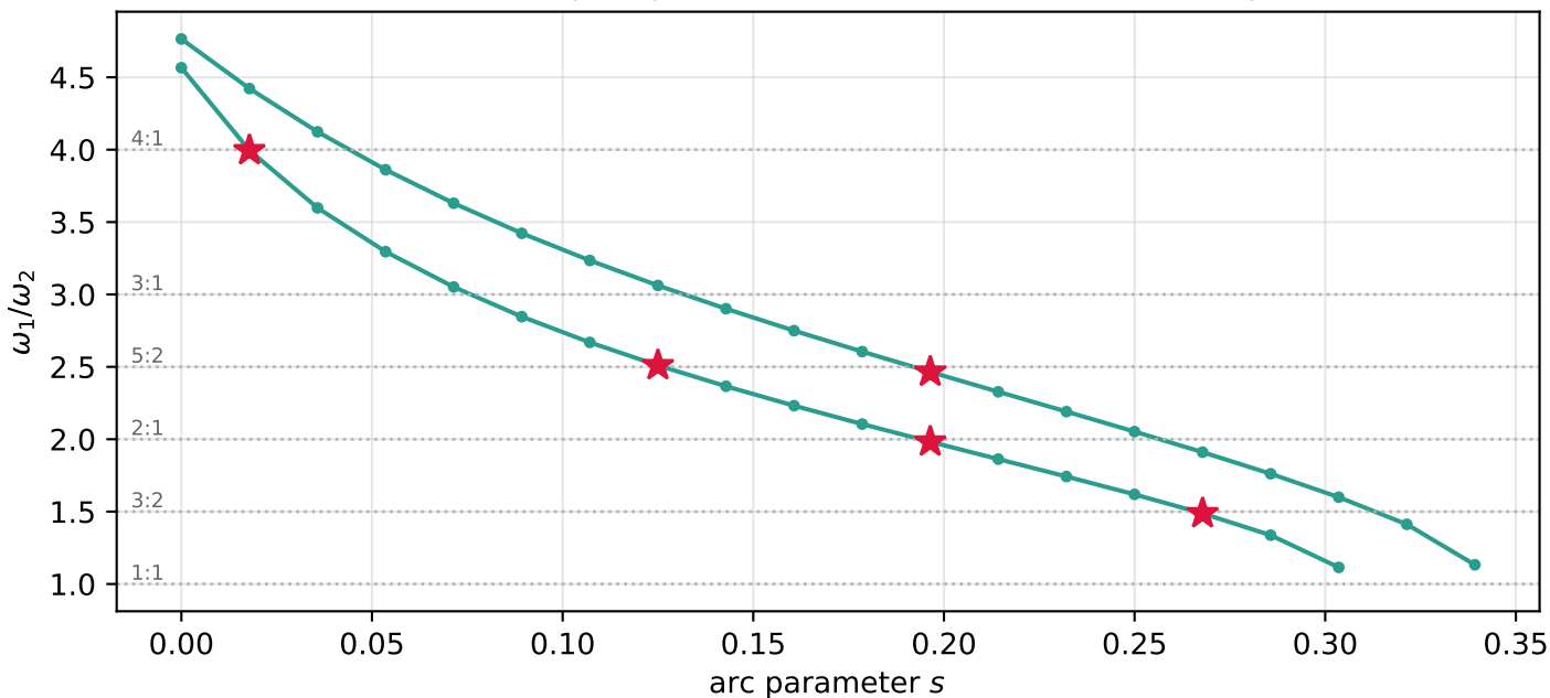
Case-2 arc: centre-frequency ratio (red star = near-commensurability indicator)
