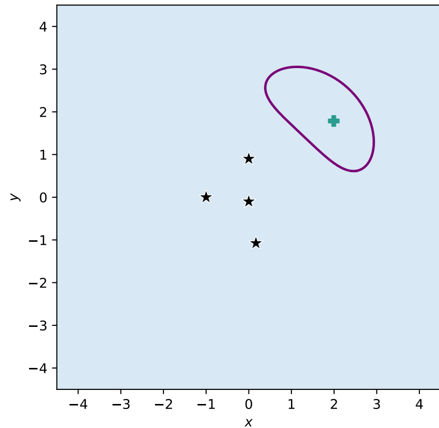
Stable orbit (fam3), C_J = 21.34 librates inside one Hill component
