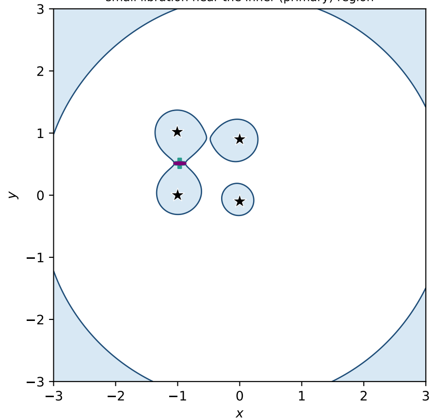
Real-unstable orbit (fam5), C_J = 13.33 small libration near the inner (primary) region
