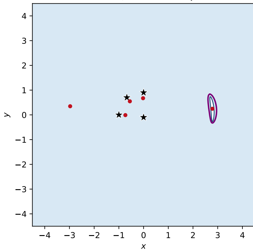
Case-1 stable regime, orbit fam2 ( C_J = 24.04 )
