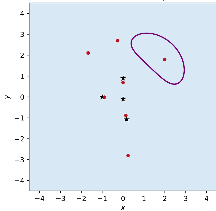
Case-2 stable regime, orbit fam3 ( C_J = 21.34 )
