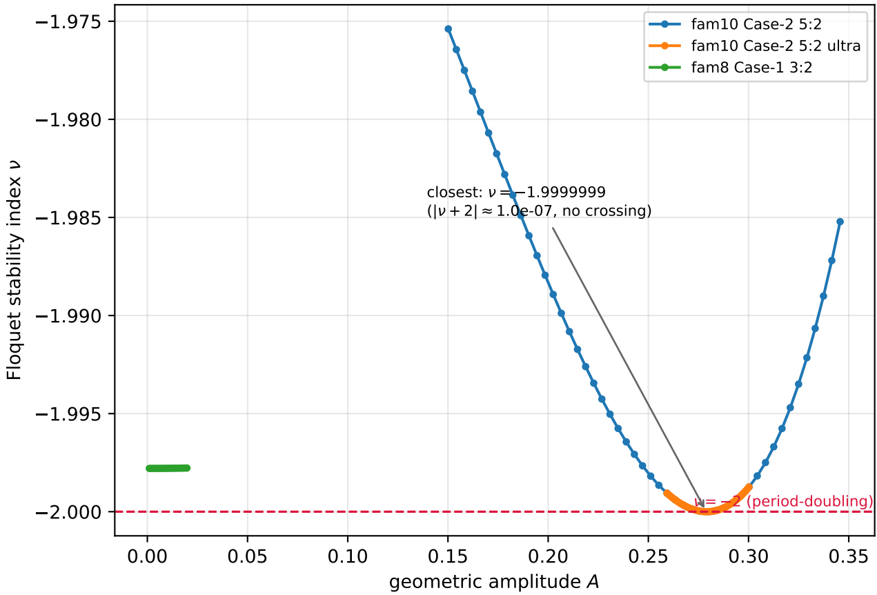
Approach to the period-doubling threshold \nu = -2 (fine scan; the multiplier stays on the unit circle)
